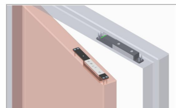
Hollow door installation
